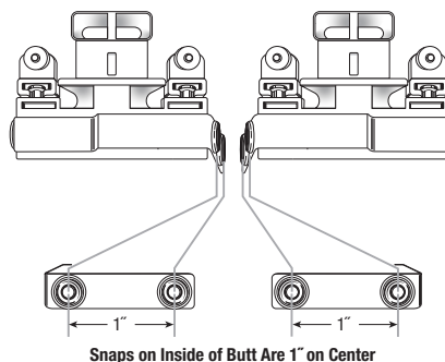
Premium Ripplefold® Butt Master
