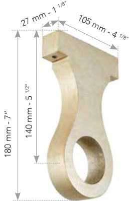
Support plafond-mur 140 mm - 5 1/2" Wall-ceiling bracket
