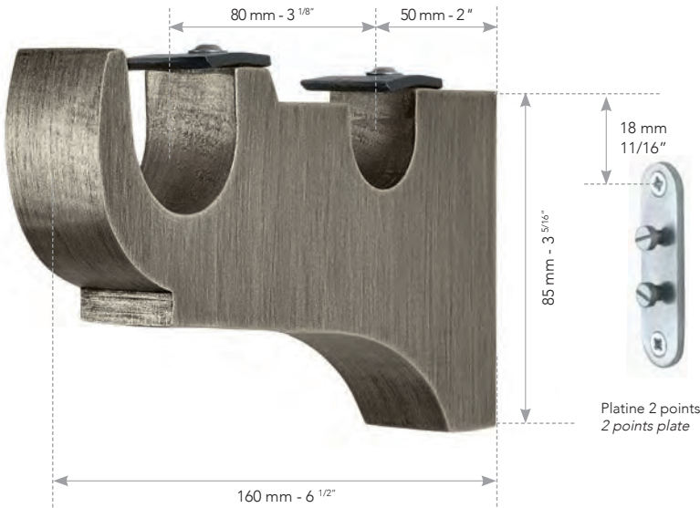
Support intermédiaire double ø 35 mm + 25 mm - ø 1 3/8" + 1" Central double bracket
