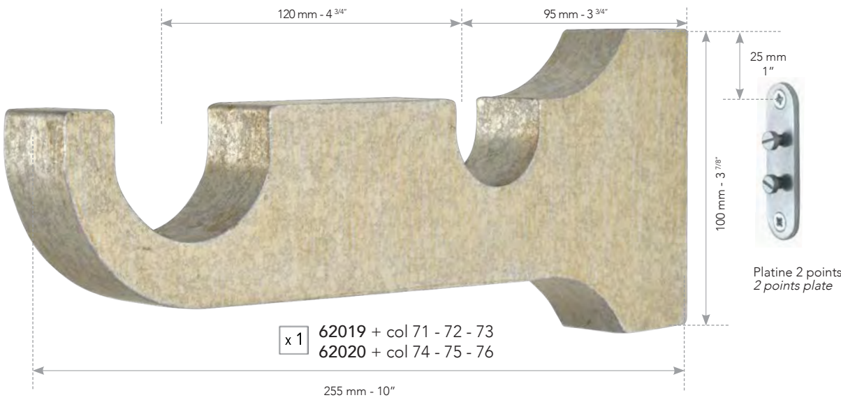
Support intermédiaire double ø 50 mm + 35 mm - ø 2" + 1 3/8" Central double bracket
