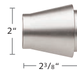
2130INC-XX Inca Finial
