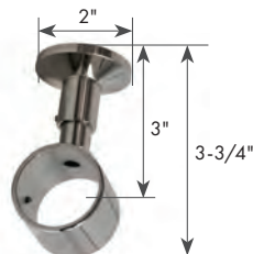
CEILING BRACKET DSG43
