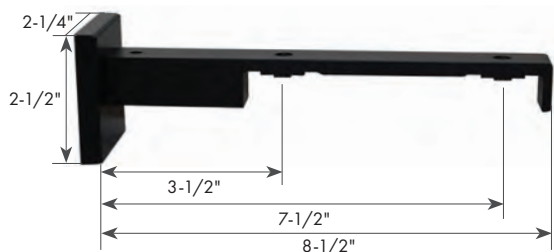
METAL DOUBLE BRACKET DIN4400
