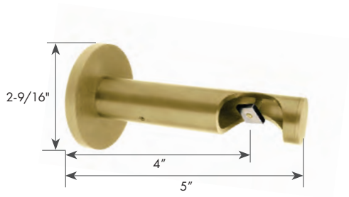
METAL SINGLE BRACKET DTR41
