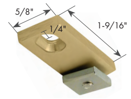
METAL CEILING BRACKET DTR44
