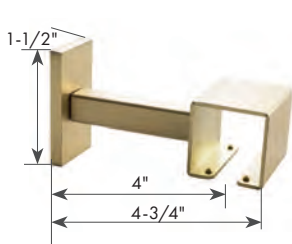
SINGLE BRACKET DCU40
