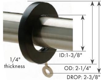
BEECHWOOD RING DTX30/BWD
