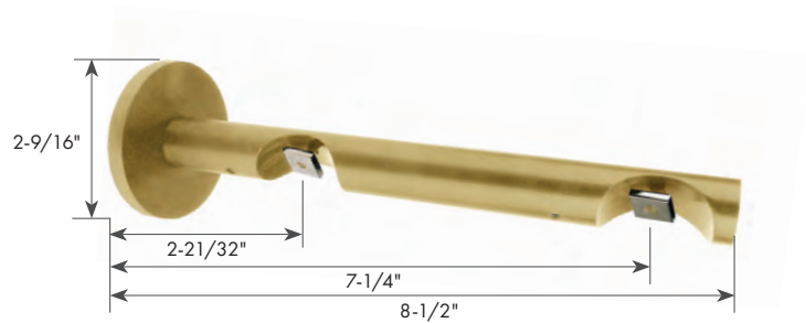
METAL DOUBLE BRACKET DTR42
