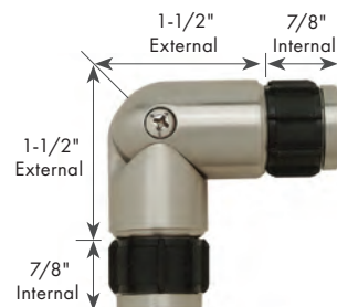
STEEL ADJUSTABLE ELBOW DTX51/STL
