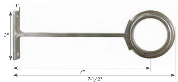
METAL WALL/CEILING BRACKET DWG47 Not available in ABZ finish.
